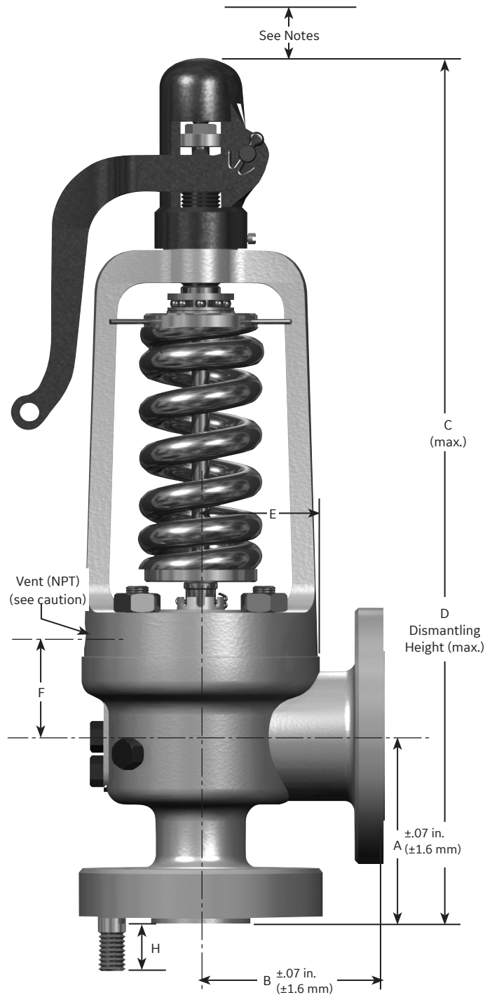
Vent and Drain Locations
