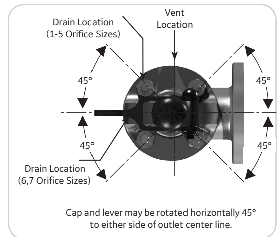
Vent and Drain Locations
