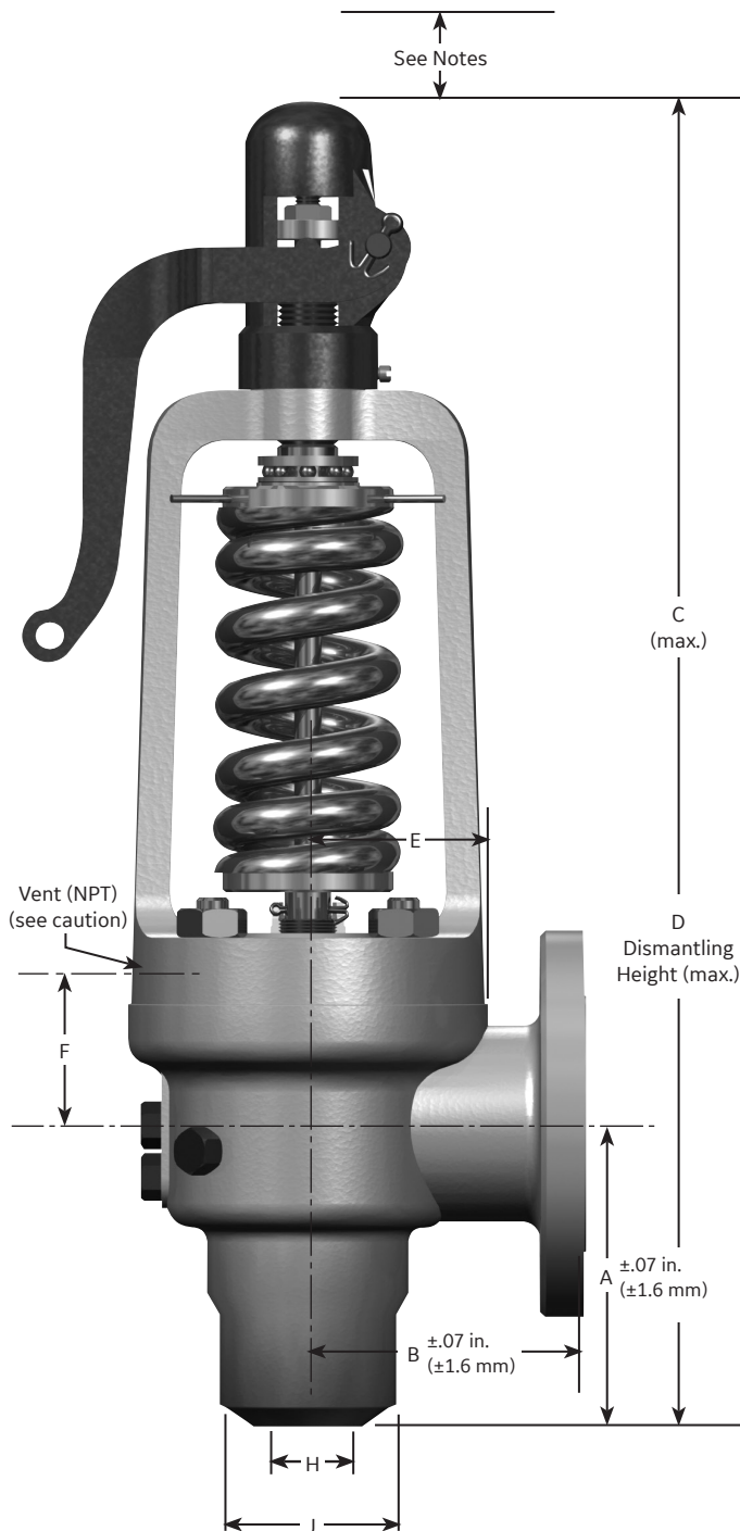
Buttweld Inlet Dimensions
