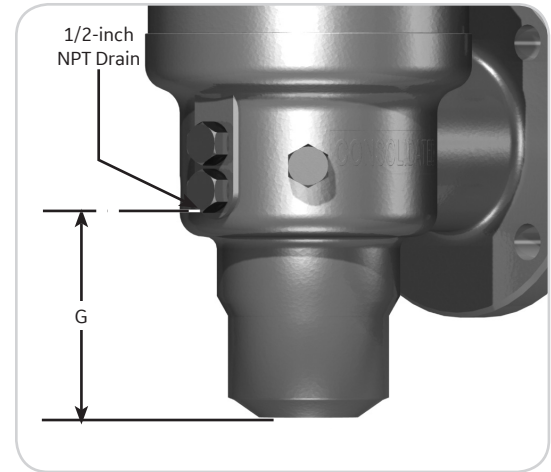
Valve General Dimensions
