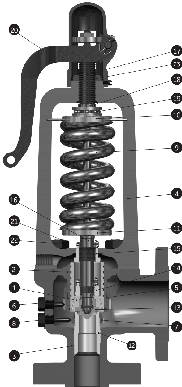
Flanged Inlet
