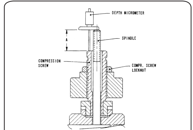
Figure 11: Compression Screw Measurement
