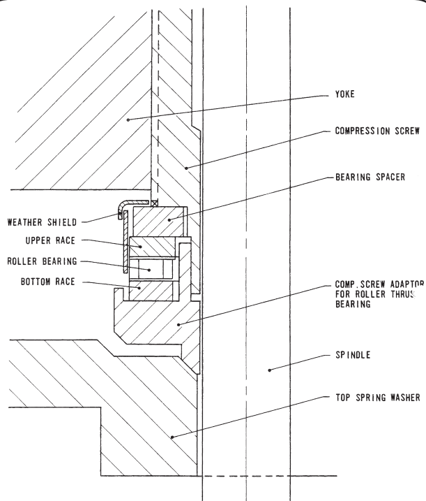
Figure 22: Roller Thrust Bearing Design
