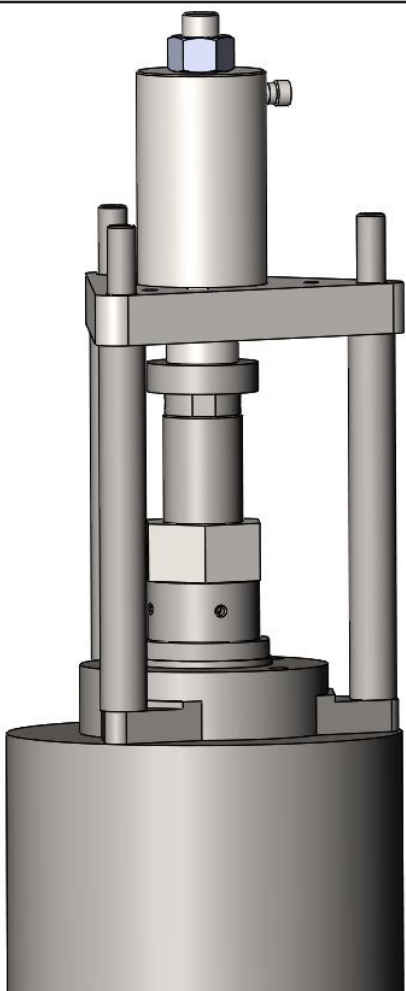
Figure 35A: Hydraulic Set Device Layout used as an Auxiliary Lift Device
