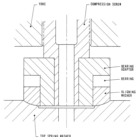
Figure 24: Garlock DU-Bearing Design
