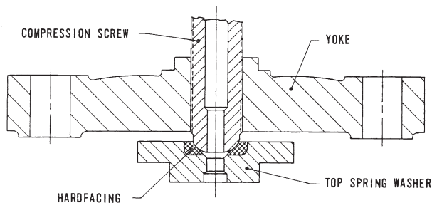
Figure 21: Spherical Compression Screw
