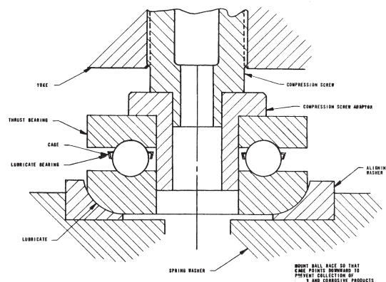
Figure 25: Ball Bearing Thrust Bearing
