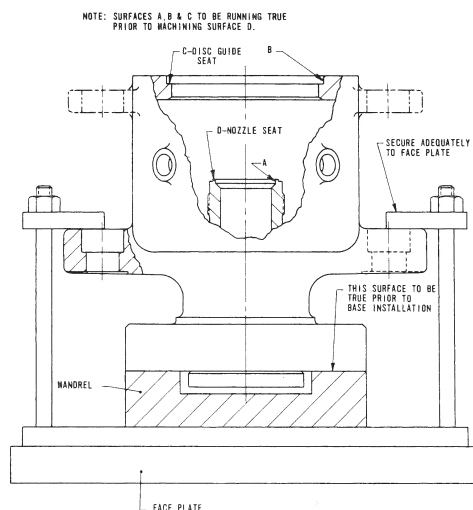
Figure 26: VTL Set-Up for Machining Base/Nozzle Assembly
