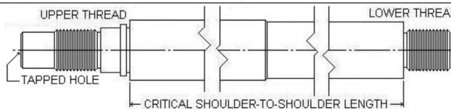
Figure X.1.18B: RT25 without Thrust Bearing Except in 3707T
