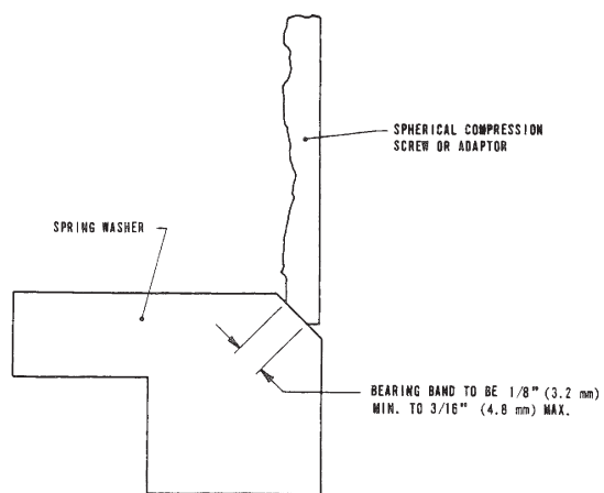
Figure 23: Spherical Radius to Spring Washer Bearing
