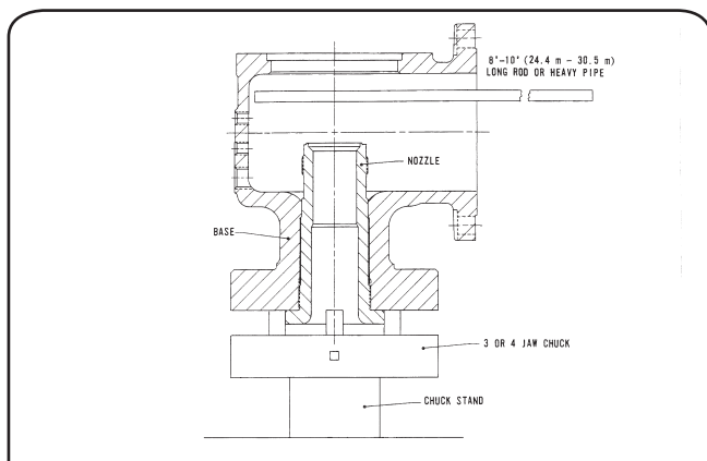
Figure 27: Nozzle Removal
