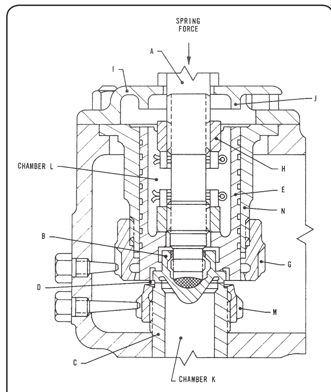
Figure 3: Valve Closed
