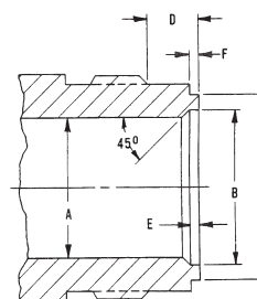
Figure 30: Machining Dimensions for Nozzle Seats
