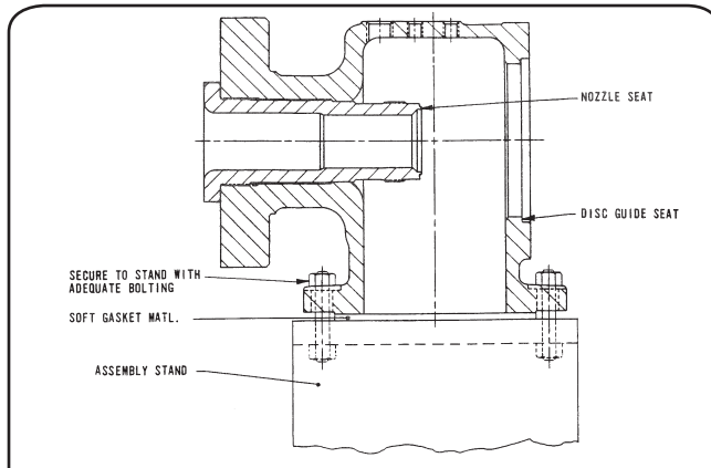
Figure 28: Nozzle Removal and Installation
