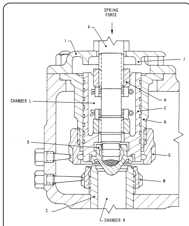
Figure 5: Valve Closing
