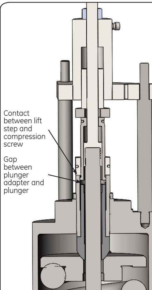
Figure 35B: Hydraulic Set Device Settings used as an Auxiliary Lift Device
