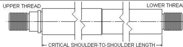
Figure X.1.18A: RT21 to RT24 & RT25 with Thrust Bearing
