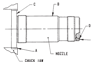
Figure 29: Lathe Set-Up for Machining Nozzle Seat
