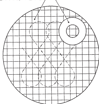
Figure 18: Lap Reconditioning
