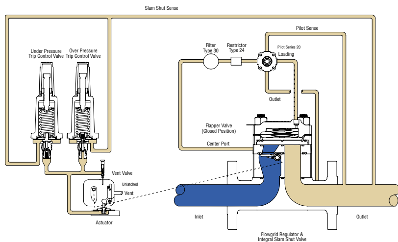
Figure 7 – Valve, Actuator & Latch Mechanism Closed
