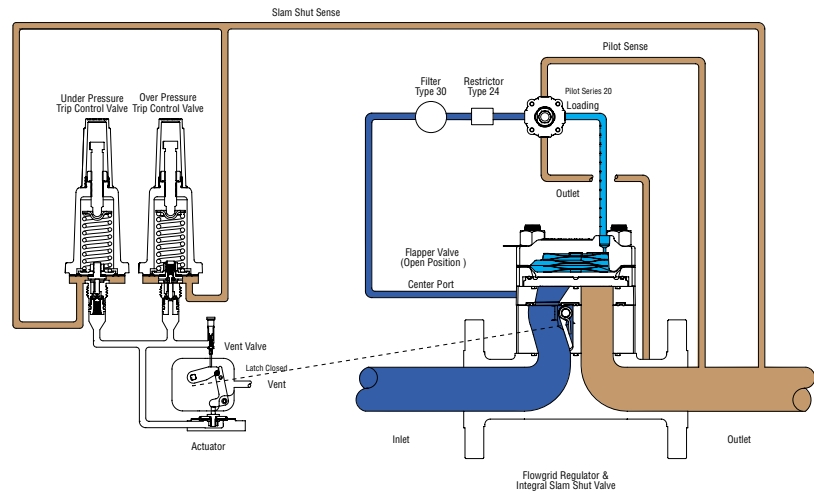
Figure 5 – Valve, Actuator & Latch Mechanism Open
